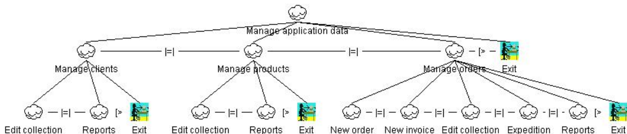
Fig. 1 Mapping of application functions onto user tasks
