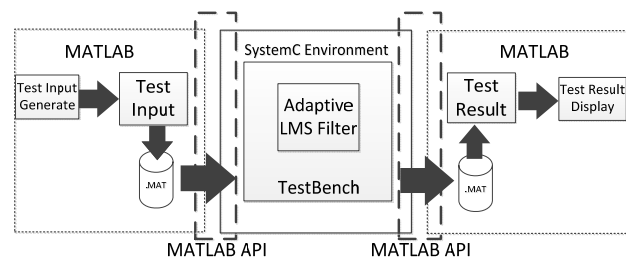
Fig. 3 SystemC model simulation flow
