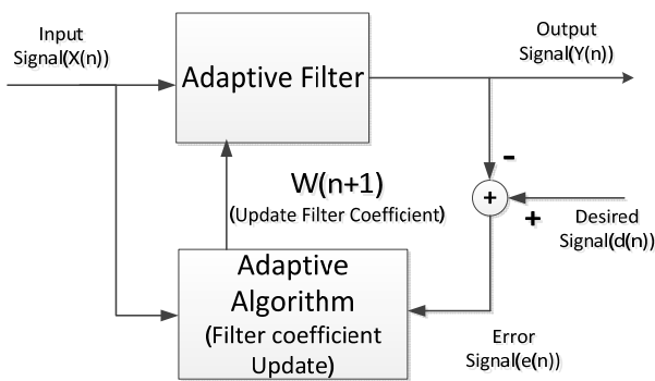
Fig. 2 Adaptive LMS filter block diagram
