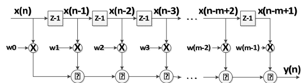
Fig. 1 Transversal Fir Filter
