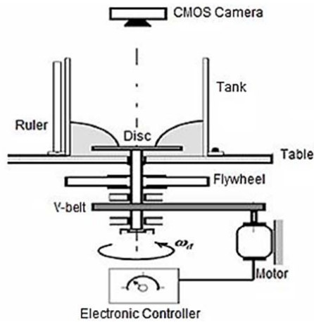
Fig. 1 Experimental setup
