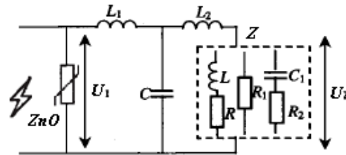
Fig. 3 Combination of MOV and low pass filter
