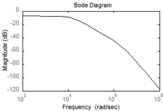
Fig. 2 1.2/50μs Surge wave frequency spectrum
