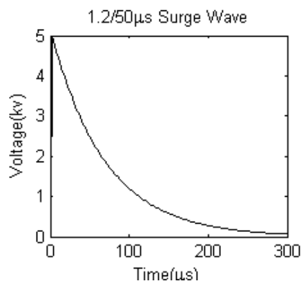
Fig. 1 1.2/50 \mu s surge wave
