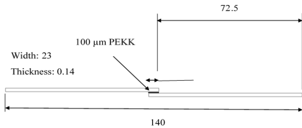
Fig. 1 Lab shear specimens (dimensions in mm)
