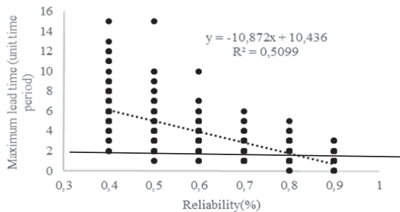
Fig. 2 Maximum lead time under different reliability
