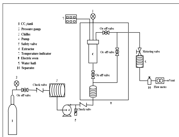
Fig. 1 Schematic diagram of SC-CO 2 extraction process
