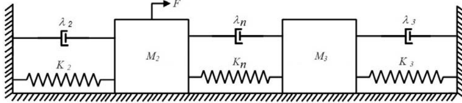
Fig. 3 Dynamical modeling of the PWCC device's structure
