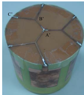
Fig. 7 Feed network of 1 × 6 array
