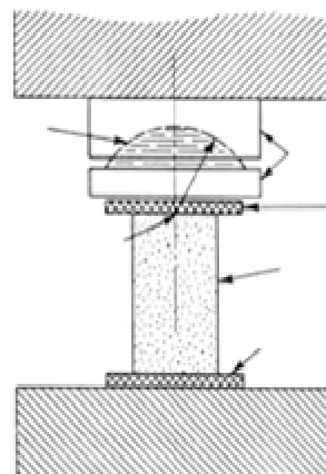
Fig. 6. Crushing Strength Tester [5]
