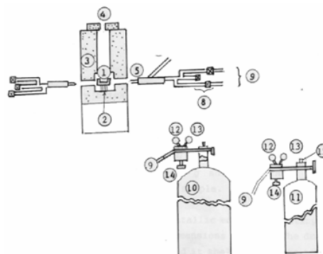
Fig. 2. Arrangement of Test Cones
