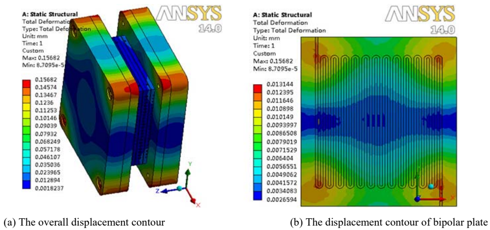
Fig. 2 The displacement contour with four locking bolts in type I
