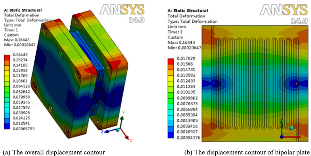
Fig. 4 The displacement contour with six locking bolts in type I
