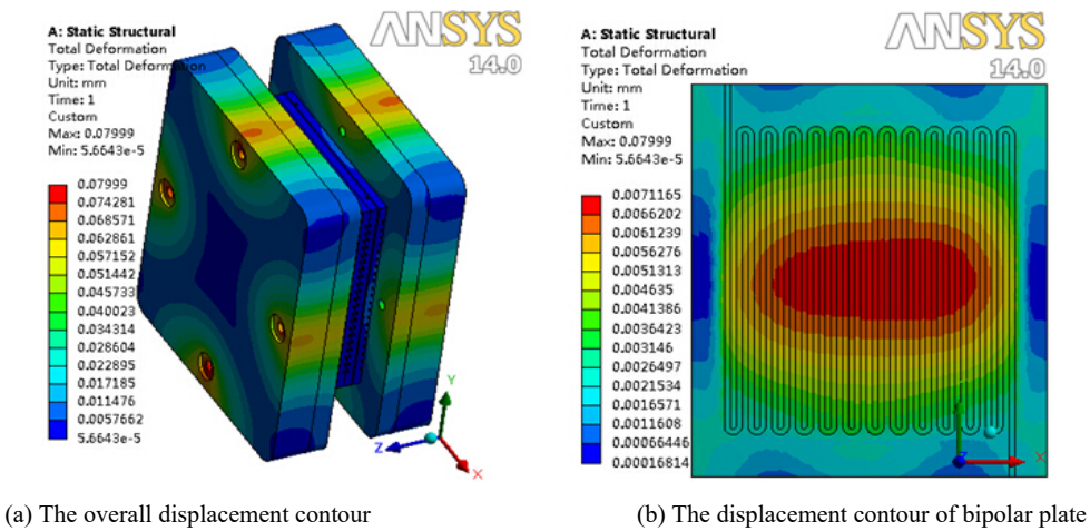
Fig. 3 The displacement contour with four locking bolts in type II
