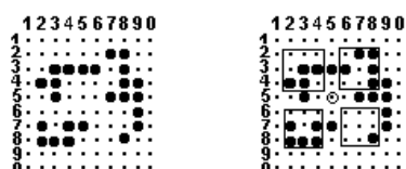
Fig. 3 a) Binary image 10×10 pixels size; b) The three layer neighborhood pixels of pixel (5, 5) on four corners
