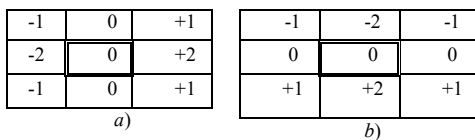
Fig. 1 Sobel operator to compute gradient component along: a) x-axis, b) y-axis.
