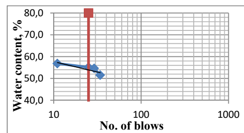
Fig. 2 Flow curve
