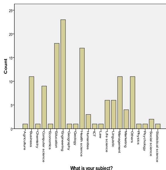
Fig. 1 Subject distribution
