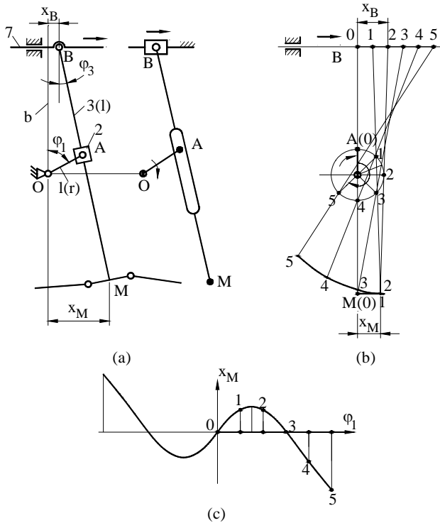
Fig. 7 The RRTR mechanism with two driving elements (RRTRT)
