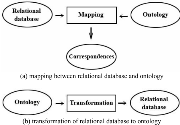
Fig. 1 Mapping vs. transformation
