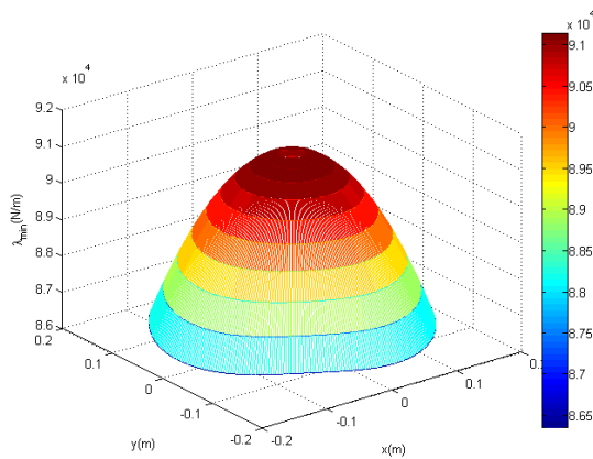
(b) Minimum stiffness map
