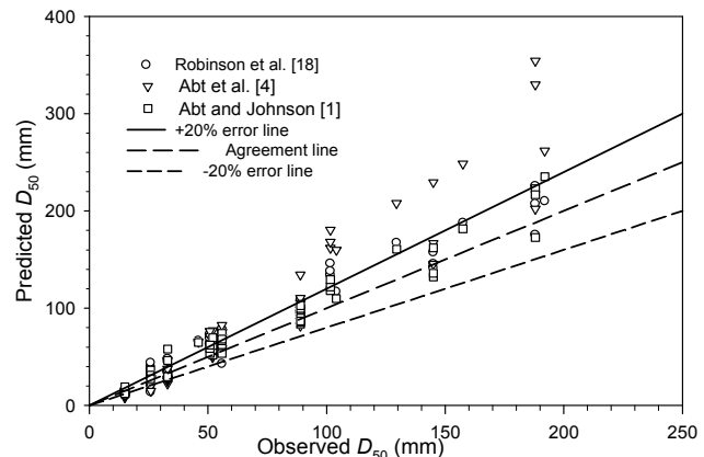
Fig. 1 Comparison of predicted D_{50} of stone using existing equation with observed one
