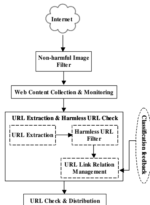
Fig. 5 Blocks for Acquiring Relevant Web Contents
