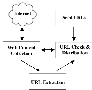
Fig. 1 Operation of the General-purpose Web Robot
