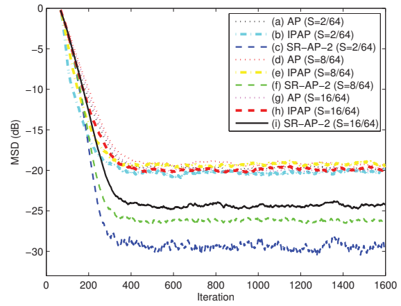
Fig. 4 MSD curves of the AP, IPAP, and SR-AP-2 algorithms for various sparsity conditions [ K = 4 , \text{SNR} = 30\text{dB} , S = 2/64, 8/64, 16/64 ]
