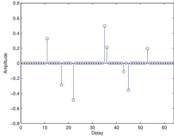
Fig. 1 Example of sparse system \mathbf{h}^o
