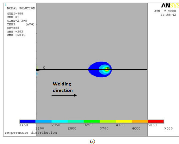
Fig. 13 Temperature profiles for three different welding speeds (a) 400mm/min, (b) 800mm/min and (c) 1200mm/min at 1800 W beam power and 85° beam incident angle – Load step no. 800
