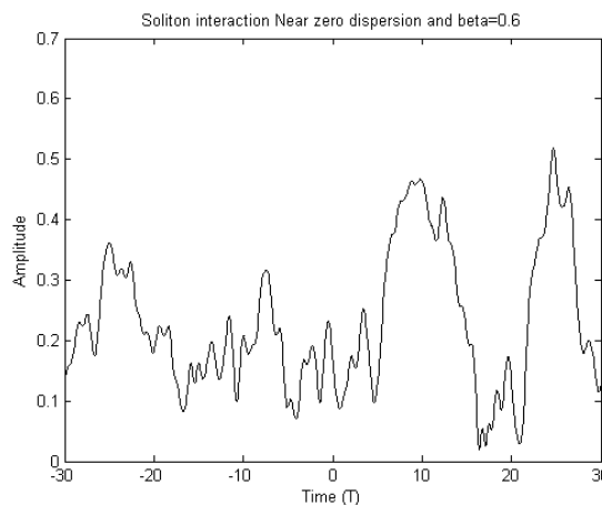
Fig. 13 Interaction between the adjacent soliton pulses at zero-dispersion wavelength with \beta=0.6 after 40 soliton periods ( Z=20\pi ).
