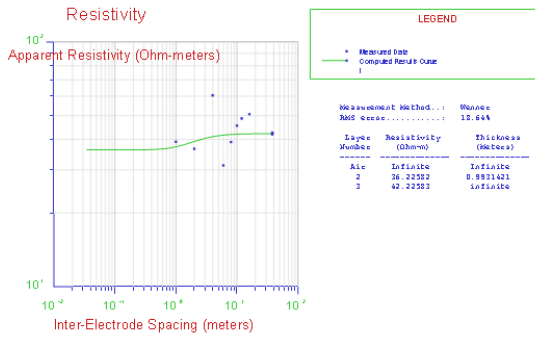
Fig. 8 CDEGS output for case study # 4
