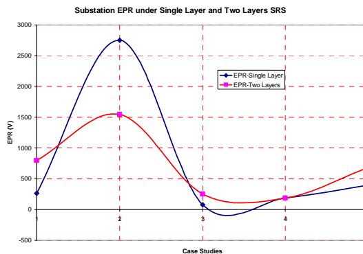
Fig. 11 Computed EPR under different soil Structure
