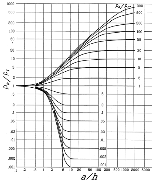
Fig. 3 Sunde's chart method to determine the two layer SRS
