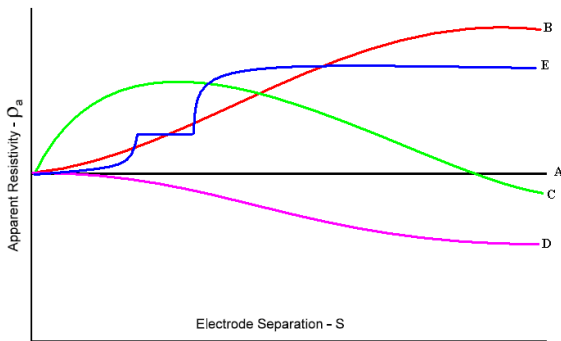
Fig. 1 IEEE 80 soil structure
