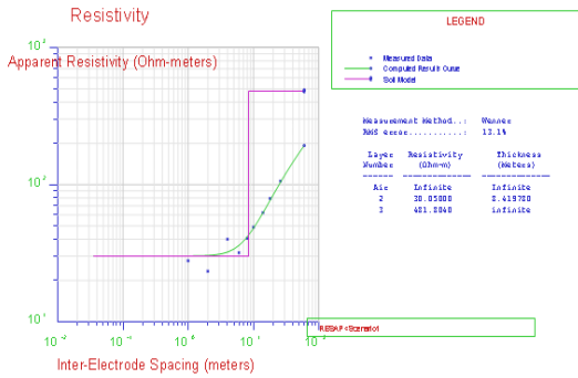
Fig. 5 CDEGS output for case study #1
