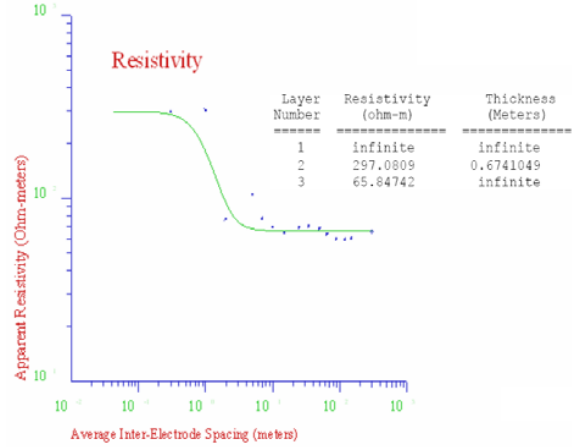
Fig. 4 CDEGS computation of the SRS
