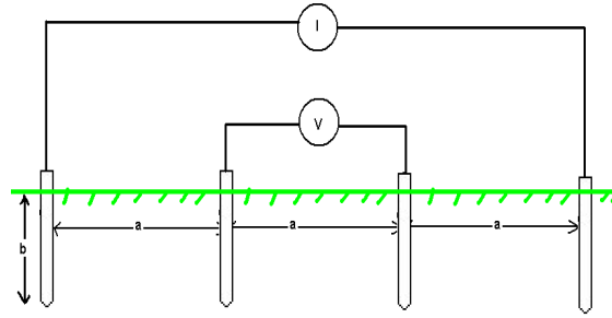
Fig. 2 Wenner Method for Soil Resistivity Test
