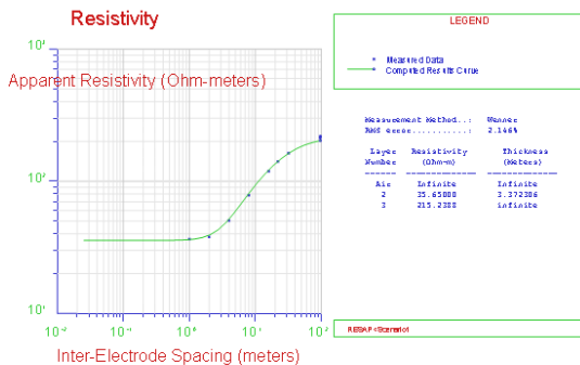
Fig. 9 CDEGS output for case study # 5
