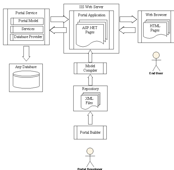
Fig. 2 System Overall
