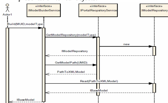
Fig. 7 Communication Diagram
