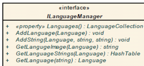
Fig. 9 Language Manager
