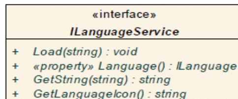
Fig. 8 Language Service
