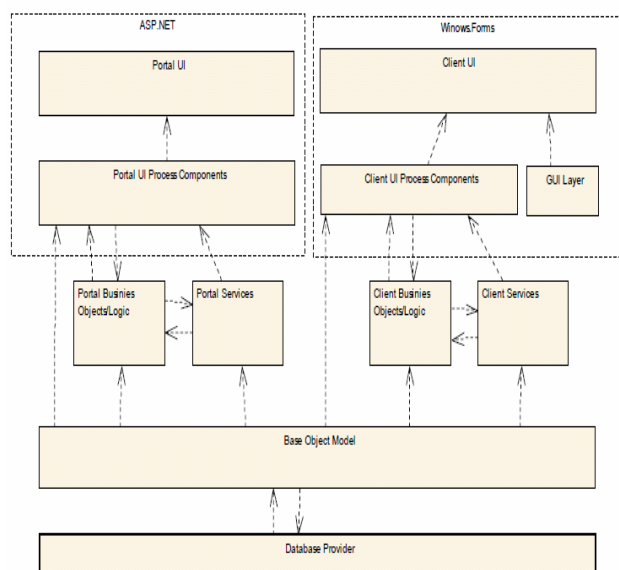
Fig. 3 Application Layers
