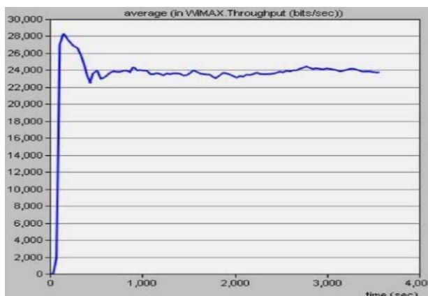
Fig. 6 Average WiMAX Throughput of Single Smart Meter
