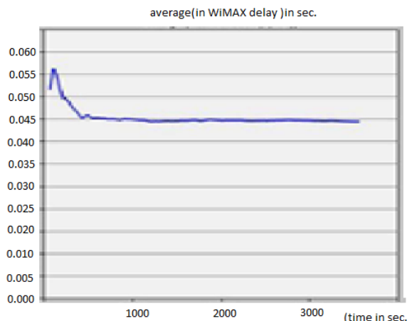
Fig. 7 Average WiMAX delay of Single smart meter
