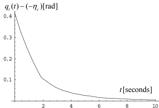
Fig. 8 Closed-loop values for q_1(t) - (-\eta_c) (forward tilting)
