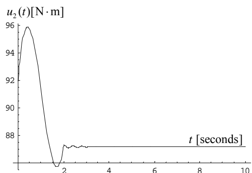
Fig. 11 Closed-loop values for u_2(t) (forward tilting)
