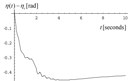
Fig. 14 Closed-loop values for \eta(t) - \eta_c (backward tilting)
