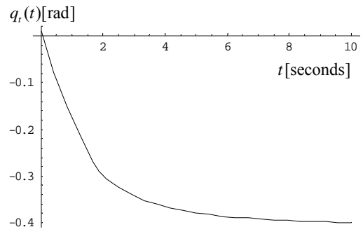
Fig. 6 Closed-loop values for q_1(t) (forward tilting)
