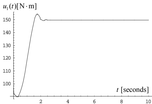
Fig. 10 Closed-loop values for u_1(t) (forward tilting)
