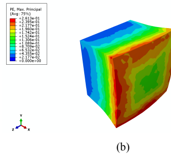
Fig. 17 Cantors of carbon composite model applied to pressure: (a) Stress, (b) Plastic strain
