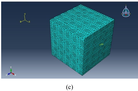
Fig. 15 Schematics of modules in simulation of non-crimp 3D orthogonal carbon fabric composite in ABAQUS: (a) Boundary conditions, (b) Tensile loading, (c) Mesh generation
