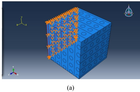
Fig. 14 Simulation of non-crimp 3D orthogonal carbon fabric composite in ABAQUS: (a) Schematic of whole structure, (b) schematic of cross section
