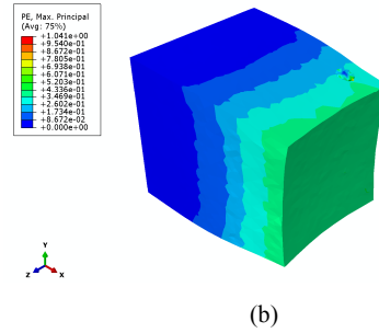
Fig. 16 Cantors of carbon composite model applied to tensile: (a) Stress, (b) Plastic strain
