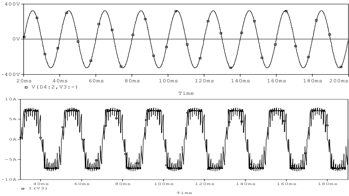
Fig. 6 Input voltage and input current waveforms of Boost PFC Converter with R Load
