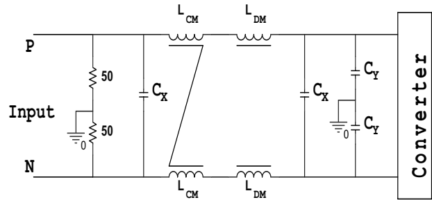
Fig. 3 EMI Filter
