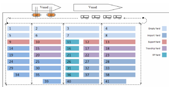
Fig. 9 SRCT Yard Layout
