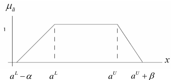
Fig. 1 Trapezoidal Fuzzy Number
