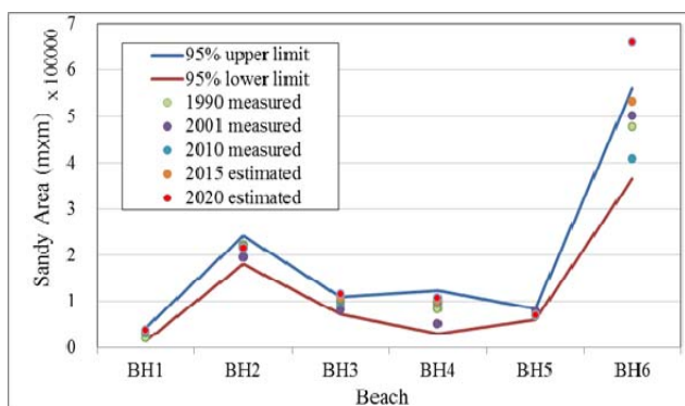
Fig. 7 Total sandy area for each beach in different years
