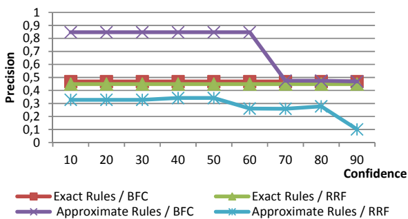
Fig. 10 Variation of precision rates associated to exact and approximate rules after partial mapping using BFC's and RRF's classification rules
