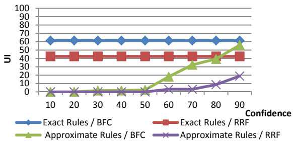
Fig. 9 Variation of UI rates associated to exact and approximate rules after complete mapping using BFC's and RRF's classification rules
