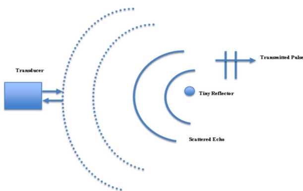
Fig. 1 Scatter Example
