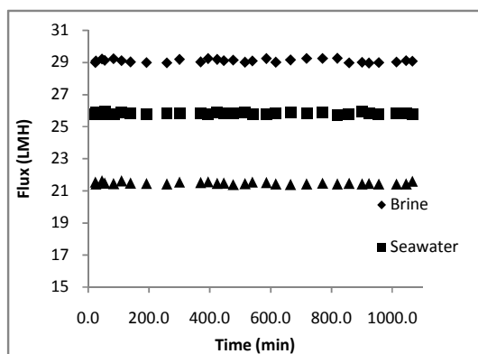
Fig. 7 Flux profile of different feed at T_i=70^\circ\text{C} , T_p=30^\circ\text{C} , Q=1.5 L/min
