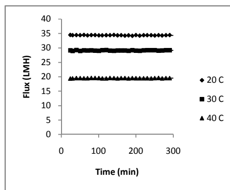
Fig. 8 Flux profile of constant feed temperature and different permeate temperature ( T_i=70^\circ\text{C} , Q=1.5 L/min, thermal brine)
