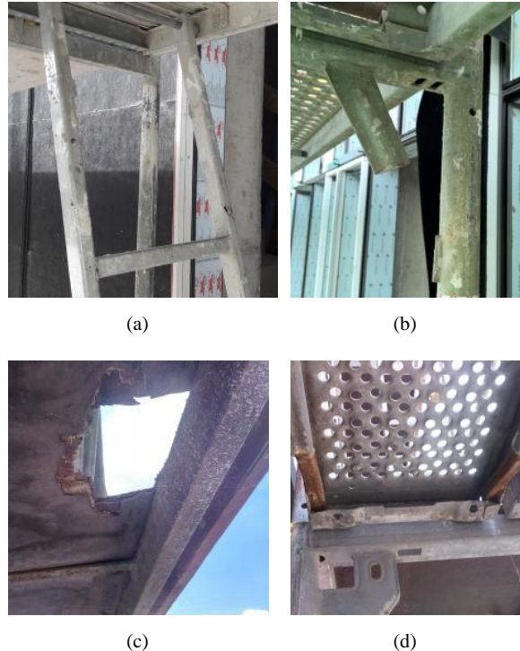
Fig. 6 Local damages; (a) no ladder step, (b) gusset plate, (c) destroyed plywood platform, (d) damage and corrosion within support of steel platform
