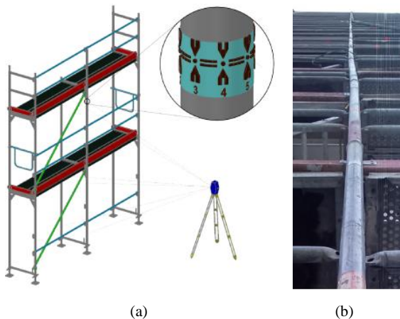
Fig. 5 Imperfections; (a) scheme of measurements, (b) sample of real imperfections
