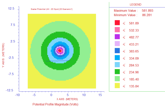
Fig. 6 Shunt Potential Magnitude
