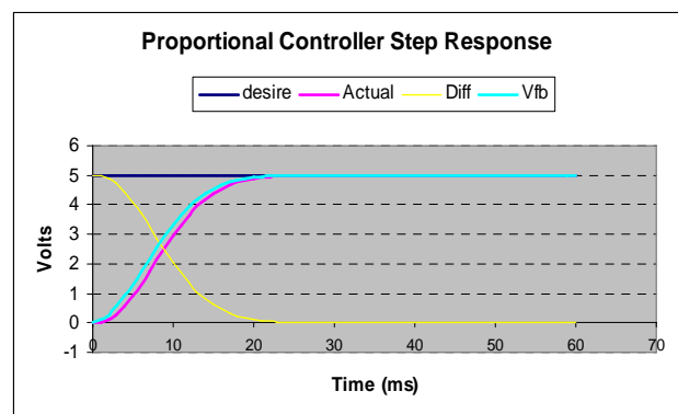
Fig. 5 Step Response of Proportional Controller
