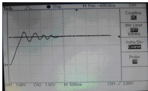
Fig. 13 Response of proportional fuzzy controller with range of 0.488 volt
