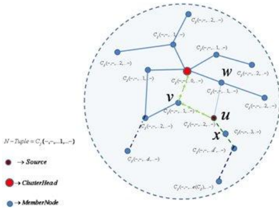
Fig. 1. Forwarding
