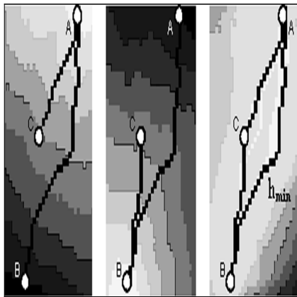
Fig. 3. Path computation
