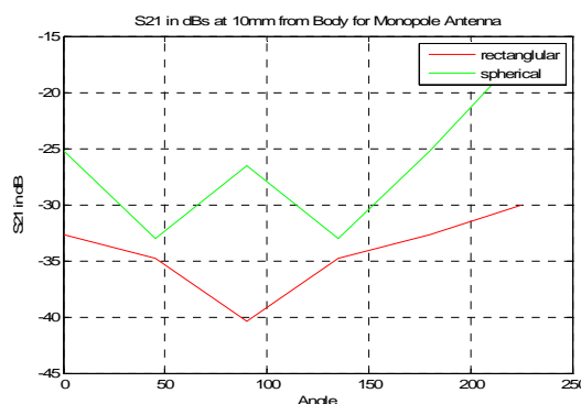
Fig. 5 Comparison of S_{21} for the spherical and rectangular bodies at the height of 10 mm.
