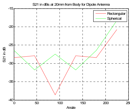
Fig. 6 Comparison of S_{21} for the spherical and rectangular bodies at the height of 20 mm.
