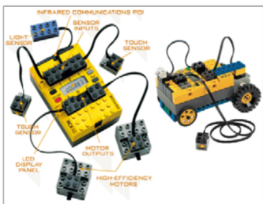
Fig. 1 RCX programmable brick
