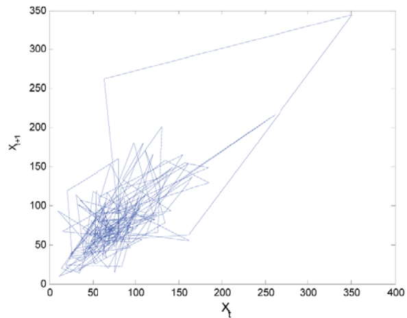
Fig. 2 Phase space
