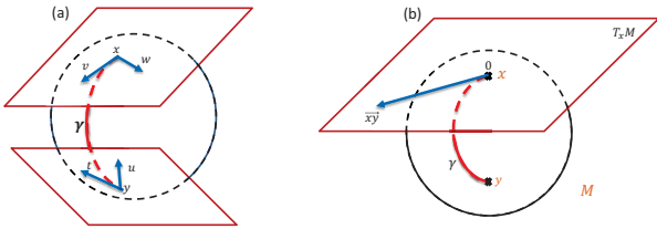
Fig. 3 (a): The tangent planes at points x and y of the sphere S_2 are different: the vectors v and w of T_xM cannot be compared to the vectors t and u of T_yM . (b): The geodesics starting at x are straight lines in the exponential map and the distance along them is conserved [2].
