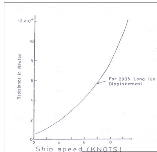
Fig. 6 resistance curve for minilace for 2951.48 t, 1 long ton = 1.016 ton
