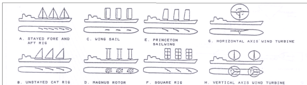
Fig. 1 Various sail rigs [19]
