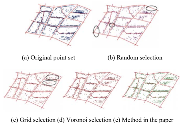
Fig. 4 Generalization Results
