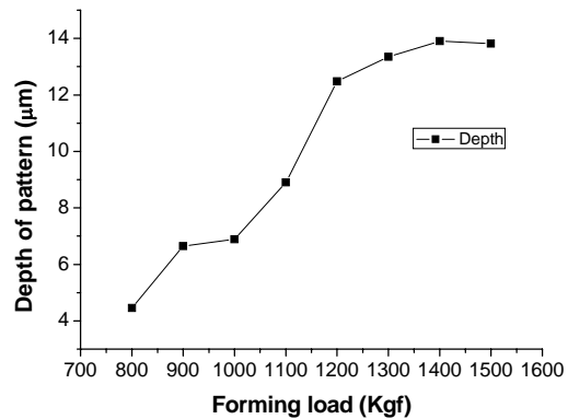
Fig. 10 Experiment result with various forming load
