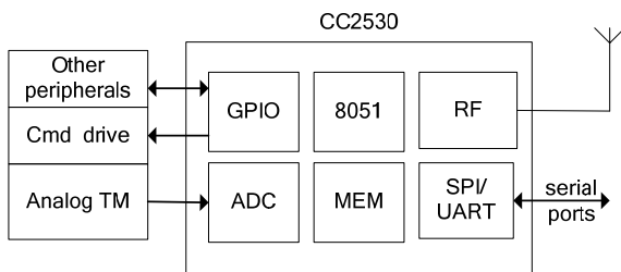
Fig. 3 Wireless node design
