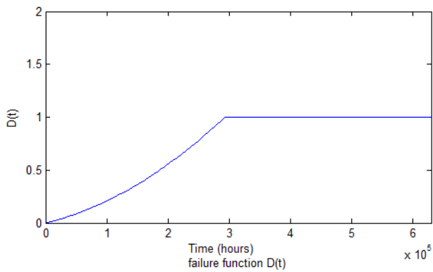
Fig. 4. Failure function.
