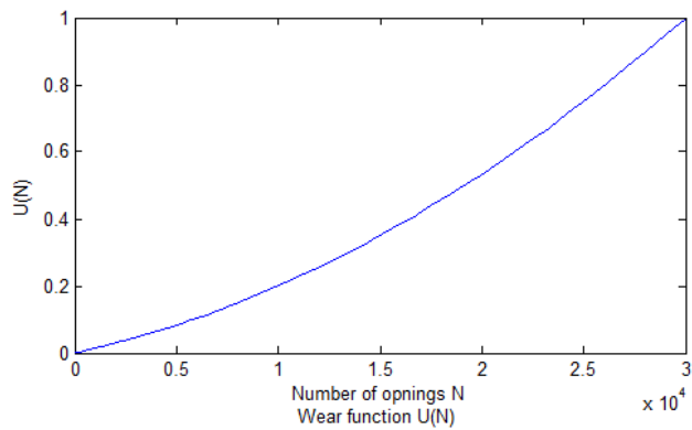
Fig. 3. wear contacts based on the number of openings.
