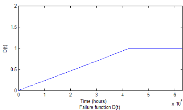
Fig. 6. Failure function.
