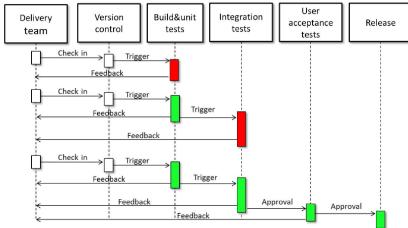
Fig. 1 Continuous Delivery Pipeline
