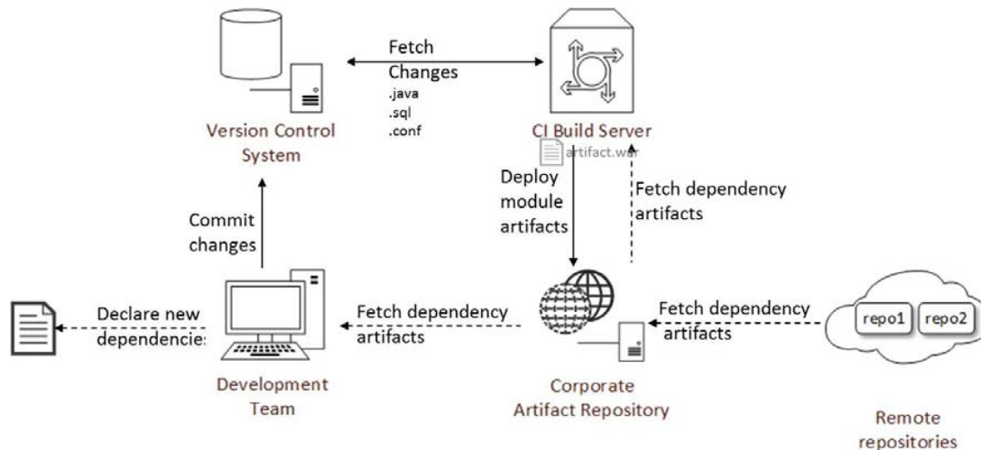
Fig. 2 Dependency Management
