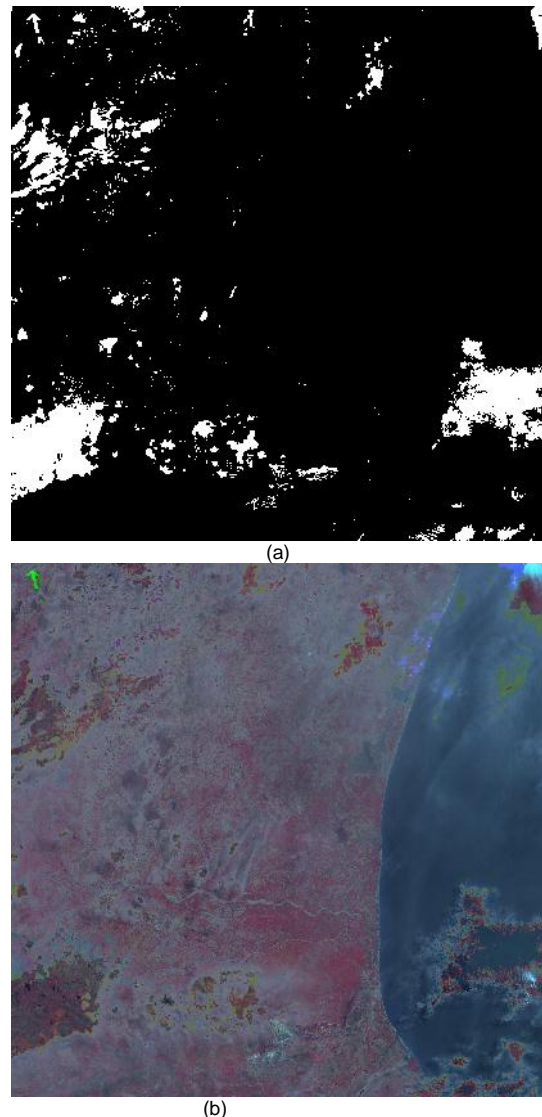
Fig. 2 Cloud detection and removal by using ABT. (a) Detected cloud area in image (26 May 2006), (b) Image (26 May 2006) after cloud removal
